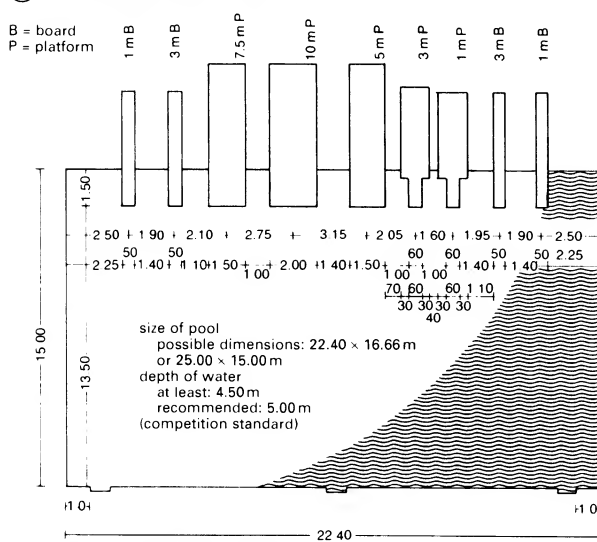
2 Diving facilities (complete): 1 to 10 m
